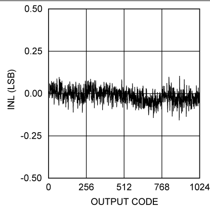
Figure 16. ADCS7477 INL
