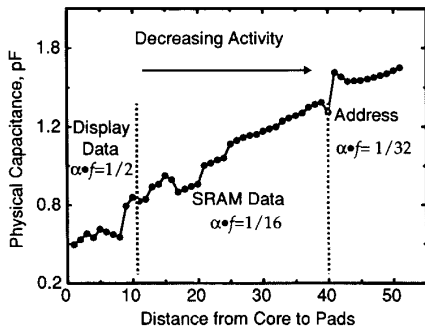
Fig. 43. Optimizing placement for low-power: Example of routing large data/control busses.
