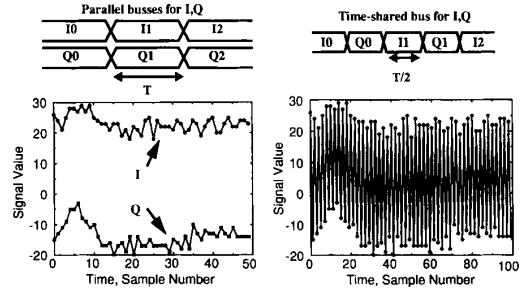
Fig. 45. Time-multiplexed hardware can increase switching activity.
