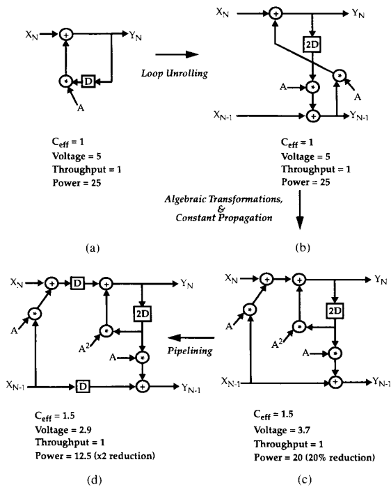
Fig. 35. Using speedup transformation to reduce power.
