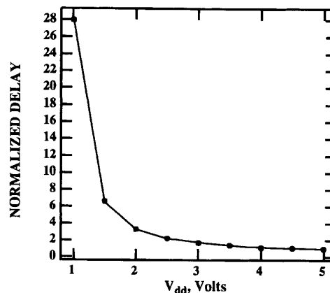
Fig. 7. Normalized delay versus V_{dd} for a typical gate in a standard CMOS process.
