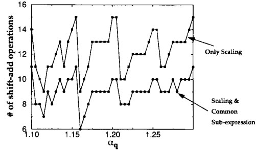
Fig. 40. Scaling and common subexpression can reduce the number of operations.
