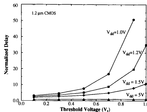
Fig. 8. Effect of threshold reduction on the delay for various supply voltages.
