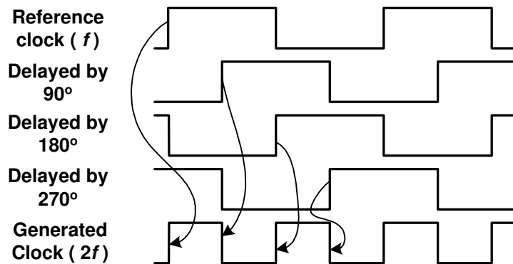
Figure 2: Example of timing for a frequency multiplier
