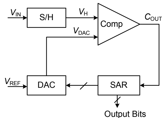
Figure 1: Block diagram of SA ADC
