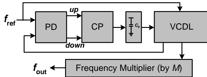
Figure 1: System Block diagram of DLL-based frequency multiplier.
