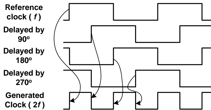
Figure 2: Example of timing for a frequency multiplier
