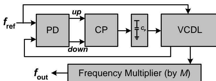
Figure 1: System Block diagram of DLL-based frequency multiplier.
