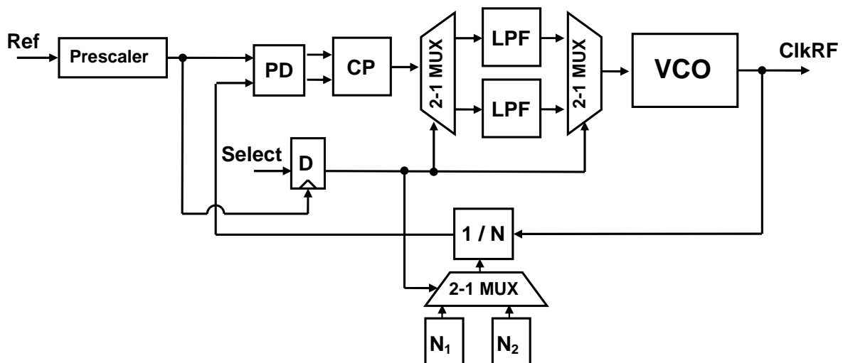
Figure 1: Block diagram of PLL-based BFSK modulator
